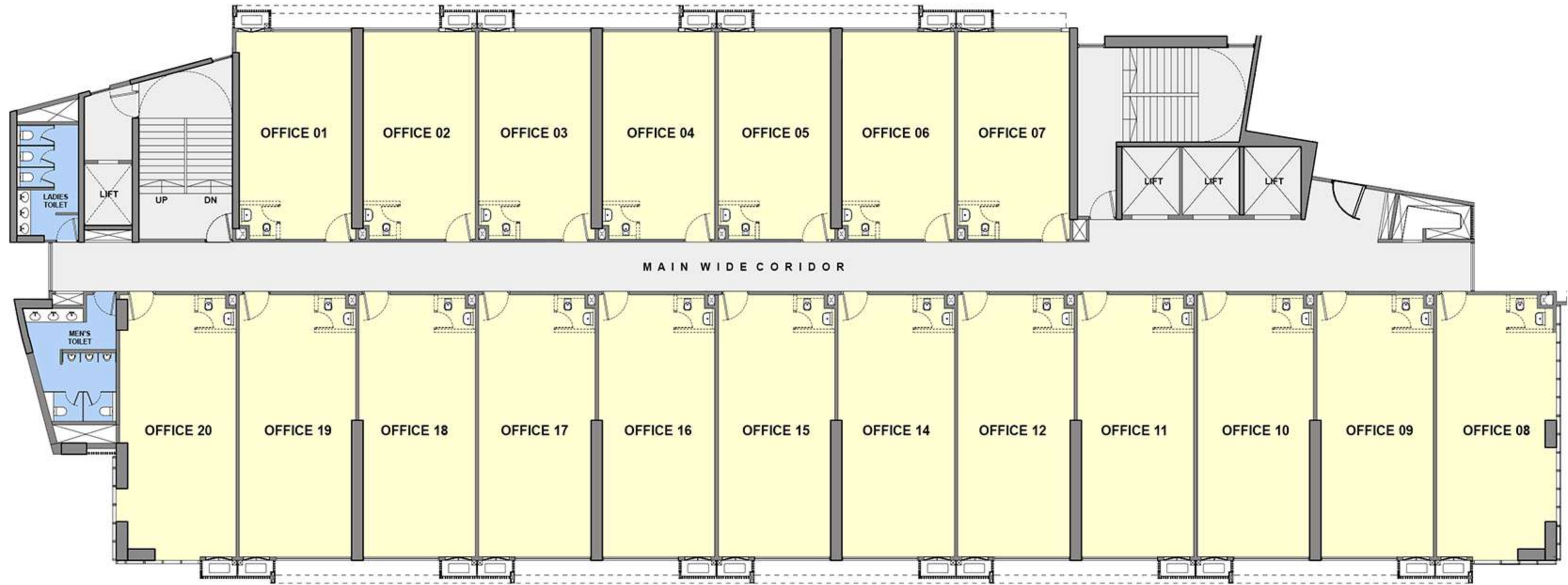
TYPICAL OFFICE LAYOUT WING B
